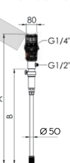
PIUSI 3.5 940
