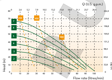
PIUSI MP 140
