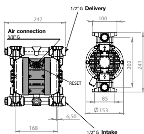
PIUSI MP 130
