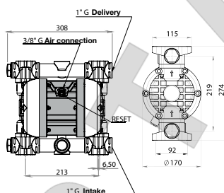
PIUSI MP 140
