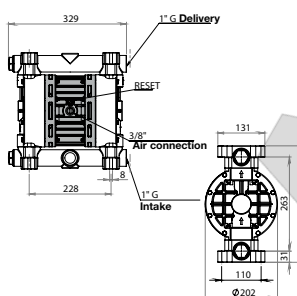
PIUSI MP 180
