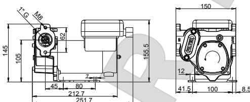
CARRY PANTHER
