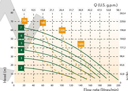
PIUSI MP 190
