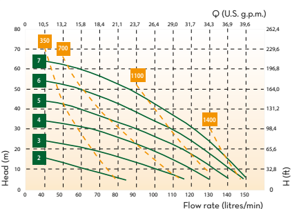
PIUSI MP 180
