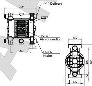
PIUSI MP 190
