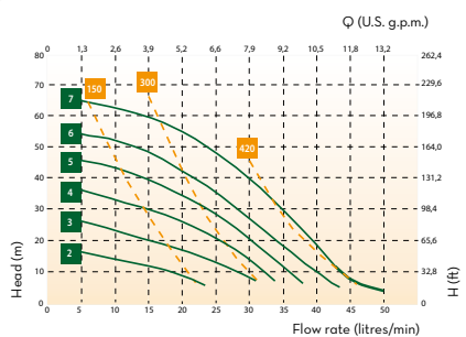
PIUSI MP 130
