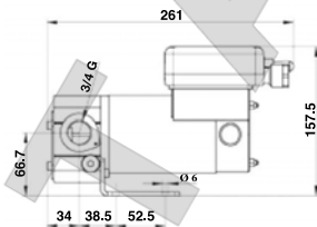
VISCOMAT DC 60/2
