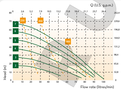
PIUSI MA 140
