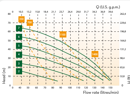
PIUSI MA 180
