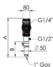
PIUSI 3.5 ST
