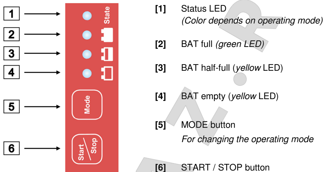
Figure 1: Control panel
